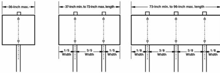
Typical Single-Post Detail Typical Two-Post Detail* Typical Three-Post Detail* (Nonbreakaway installation)
